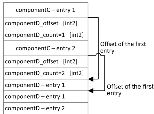
Figure 10. Template of embedded components
