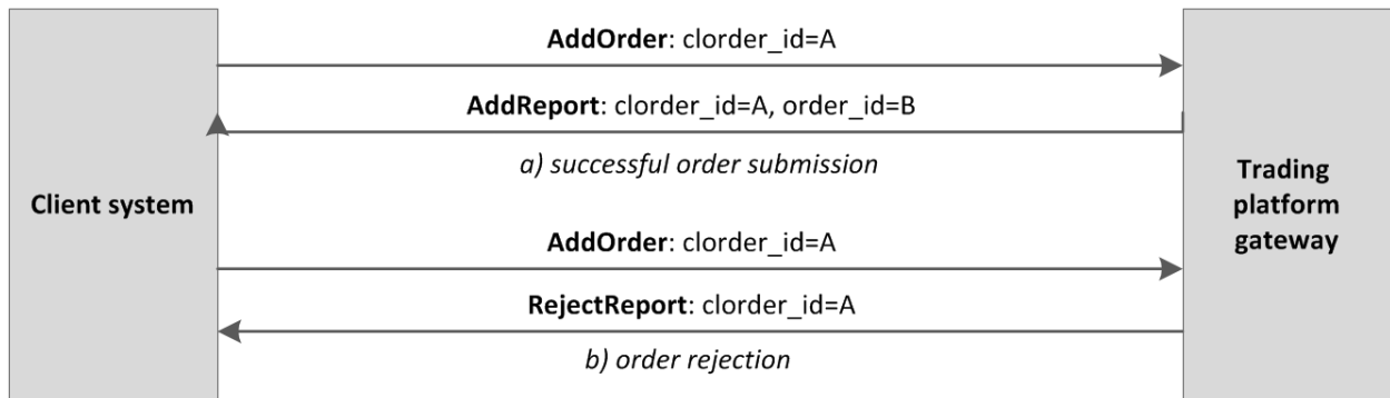
Figure 1. Order submission
